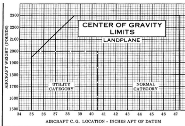
Figure 6-8. Center of Gravity Limits
